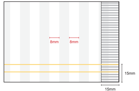
Bottom End Hem Detail
